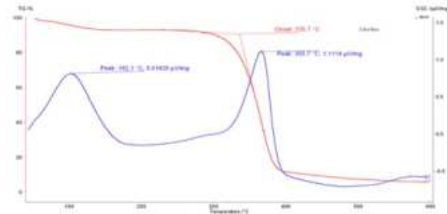
Figure 5. : Simultaneous thermal analysis (TG and DSC) of cotton fibres
