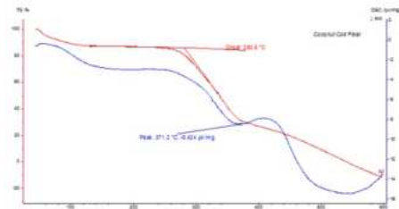
Figure 3.: Simultaneous thermal analysis (TG and DSC) of coconut coir Fibres
